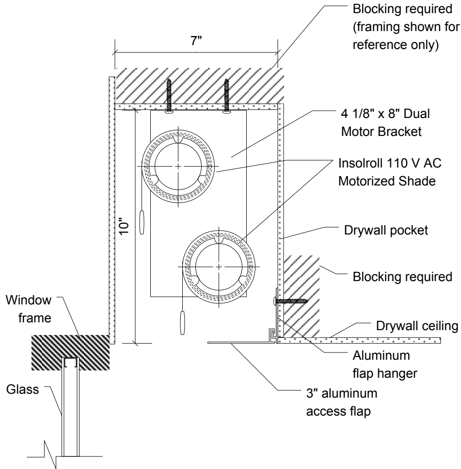
Dual 110 V AC Motorized Shades In Site-built Pocket
